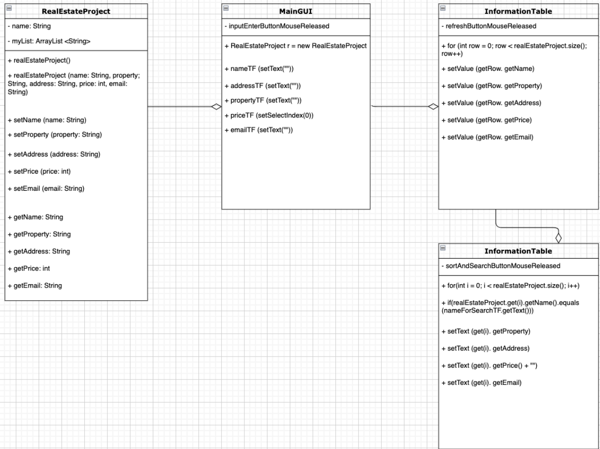
Figure 1: RealEstateProject class
